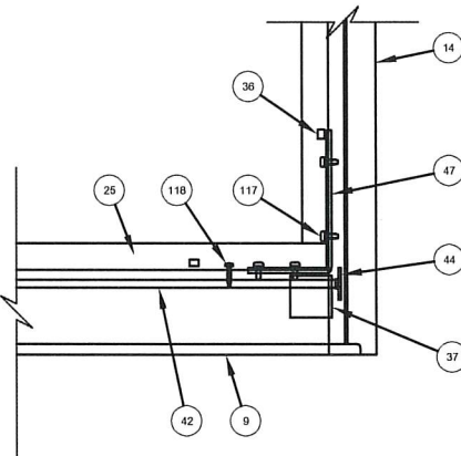
Sidelite Bottom Nose Corner
