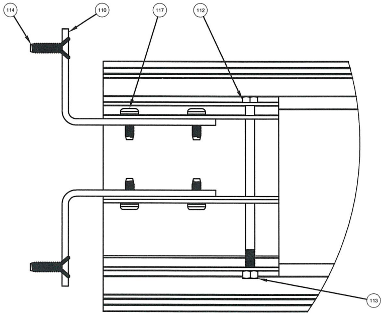
Bi-Part 4-Point Lock
