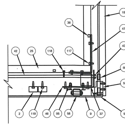
Active Leaf Bottom Nose Corner
