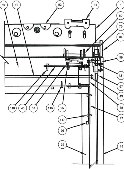
Active Leaf Top Nose Corner
