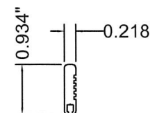
3 Sweep Housing 6063-T5
