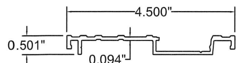
7 Threshold 6063-T6
