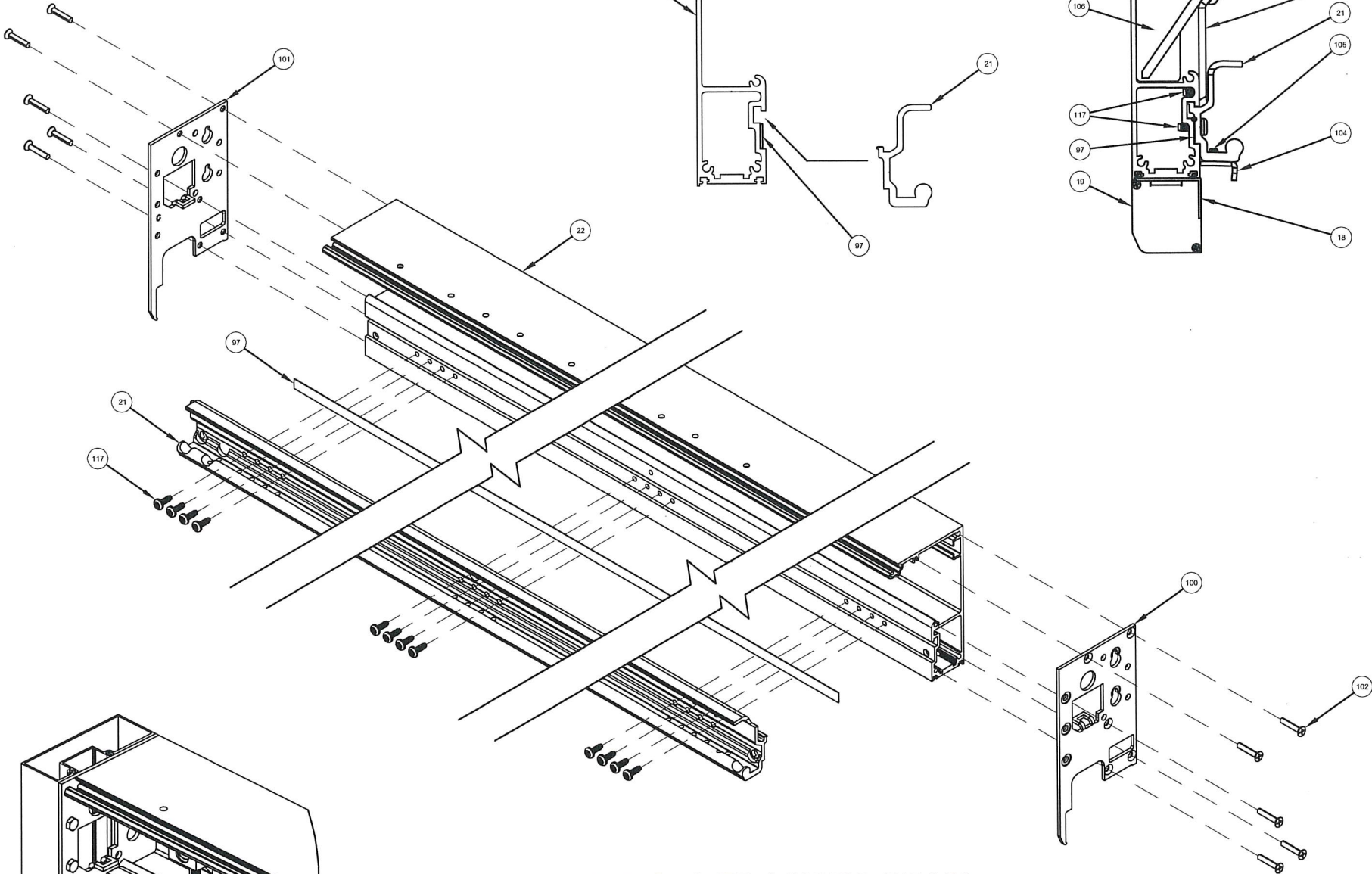
TYPICAL TRACK TO BEAM
