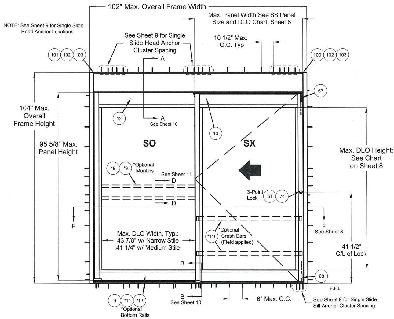
LH FSL (2 PANELS, LEFT-HAND FIXED SIDELITE)
