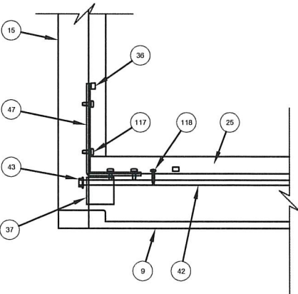
Sidelite Bottom Heal Corner
