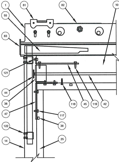
Active Leaf Top Heal Corner
