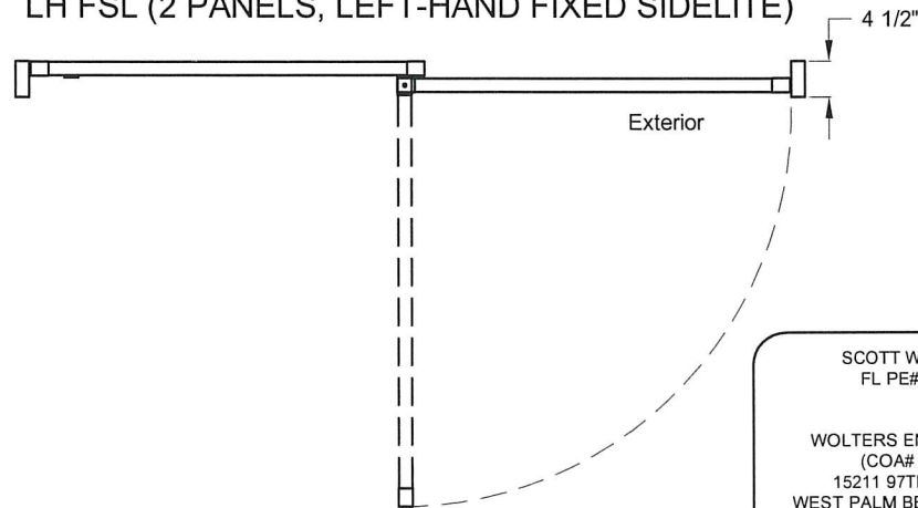
LH FSL (2 PANELS, LEFT-HAND FIXED SIDELITE)
