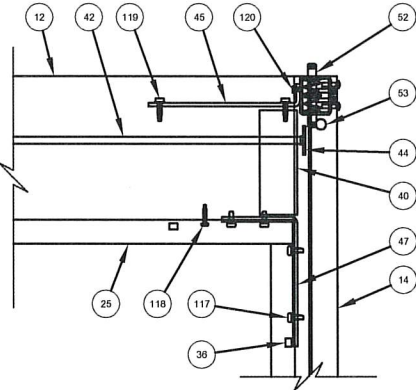
Sidelite Top Nose Corner
