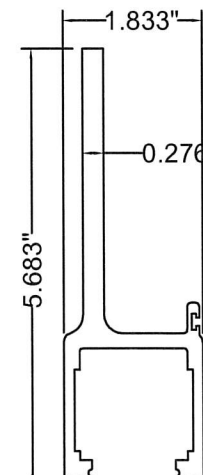
1 Carrier 6063-T6
