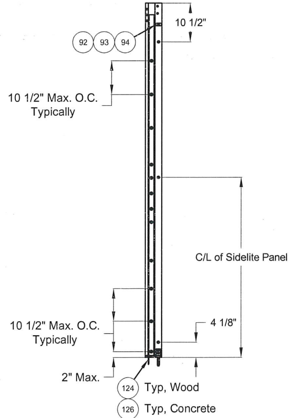
SIDELITE JAMB (Typ. both Jambs)
